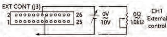
External Voltage Control of the output ※ Use a shielded cable or twisted pair wires for this control.
