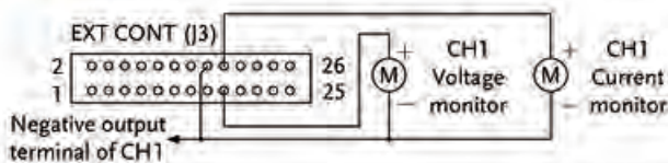
External Voltage Monitor of the Output
